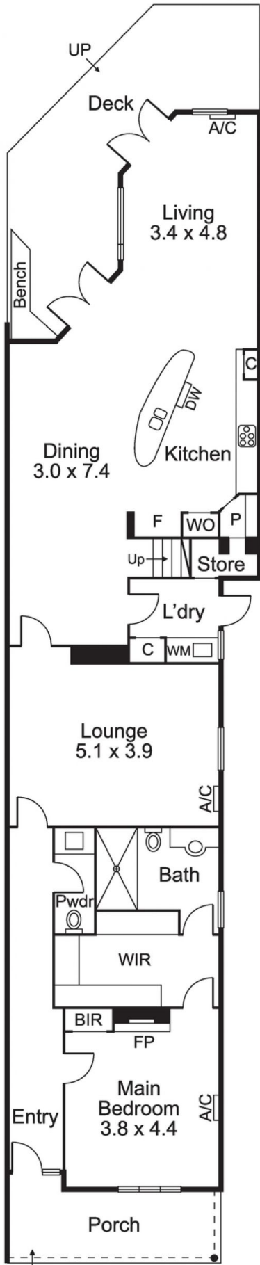
GROUND FLOOR
