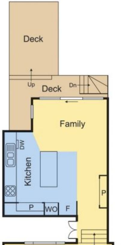
LOWER FLOOR
